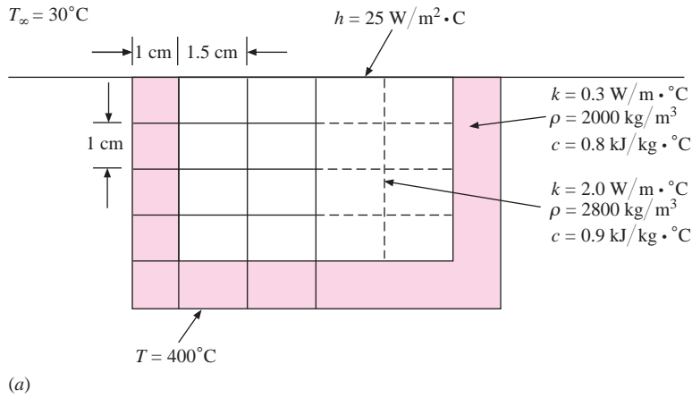
Figure Example 3-9 | (a) Physical system, (b) nodal boundaries.
